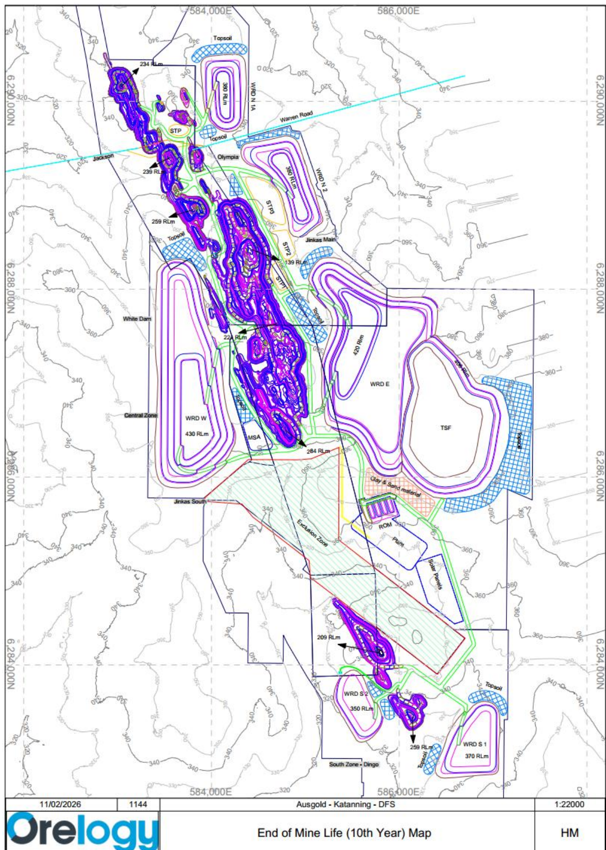
Figure 2-3: Proposed Ultimate Site Layout
