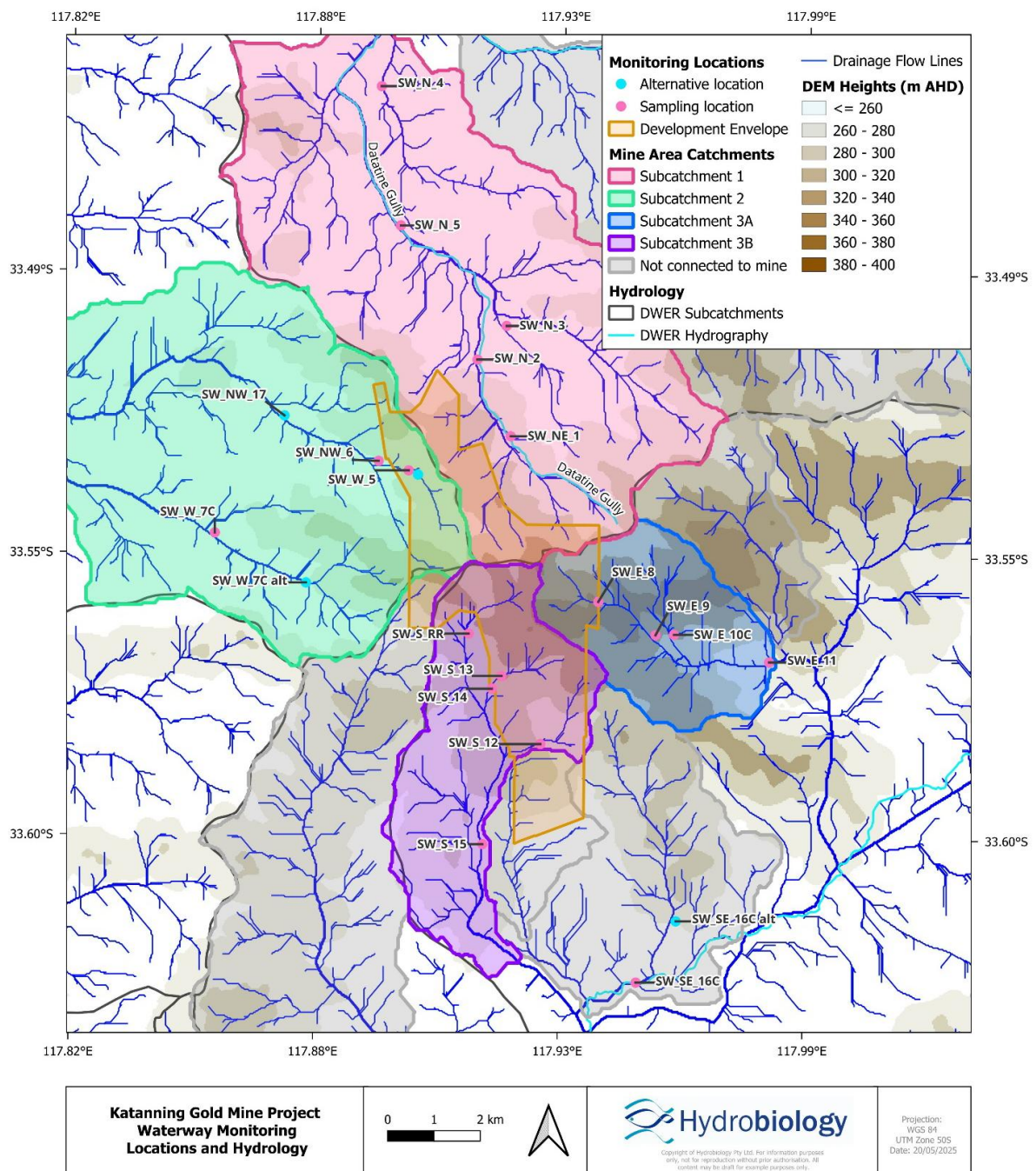
Figure 7-5: Background Hydrology and Drainage and Monitoring Sites
