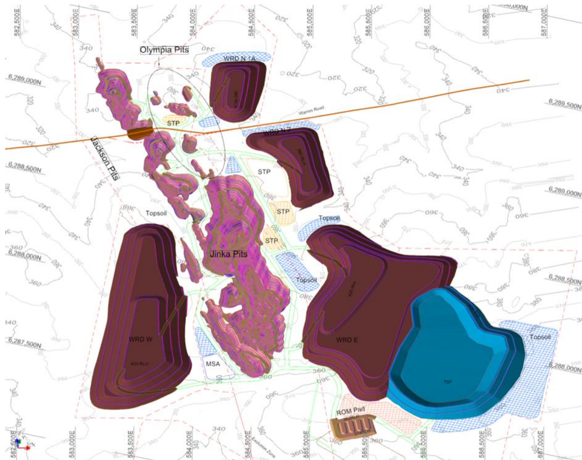
Figure 2-4: Central Zone WRL Design and Overall Layout
