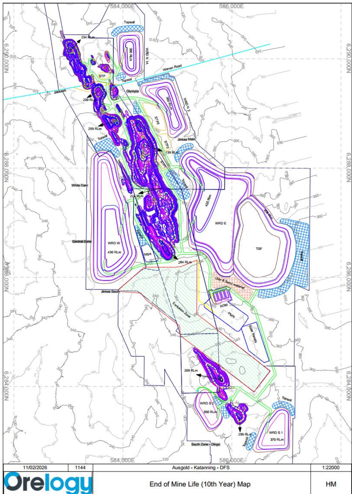
Figure 3-1: Proposed Site Layout and Location
