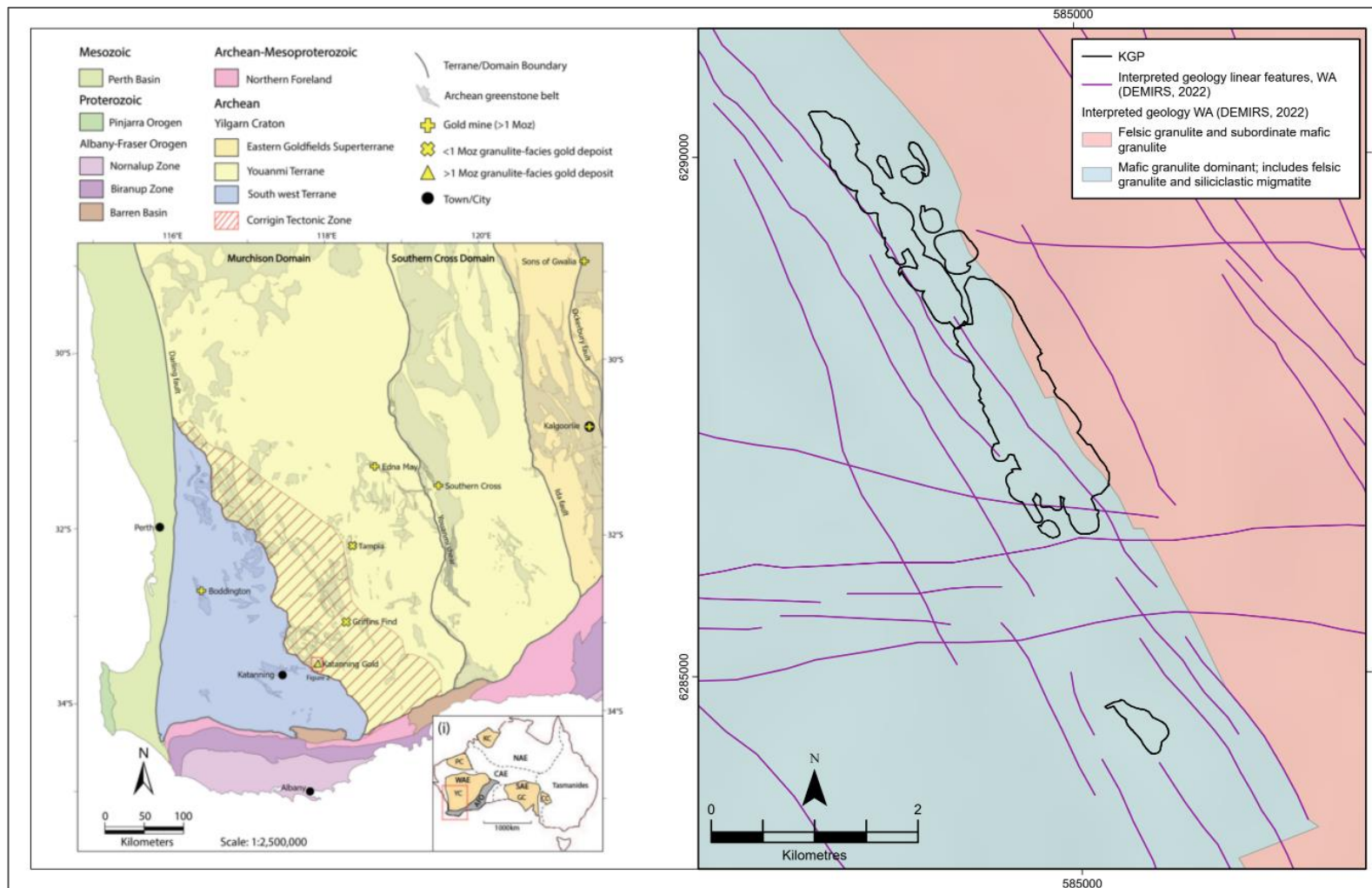
Figure 2.2: Regional geology
